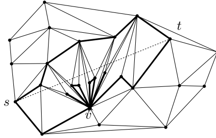
Figure 6: The graph T_{st} (shaded).
