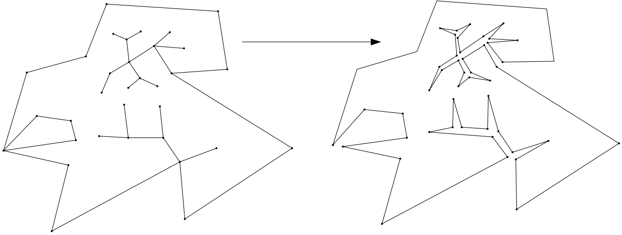
Weakly simple to simple polygon transformation
