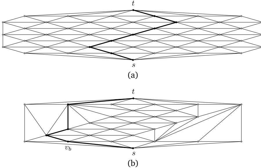
Figure 1: (a) The triangulation T with the path found by \mathcal{A} indicated. (b) The resulting triangulation T' with the “almost-vertical” path shown in bold.
