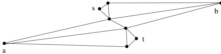
Figure 2: The ears s and t partition P into an upper and lower chain.
