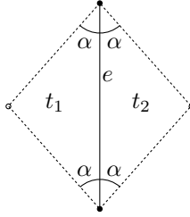
Figure 5: The edge e satisfies the diamond property if at least one of t_1 and t_2 does not contain any point of V in its interior.
