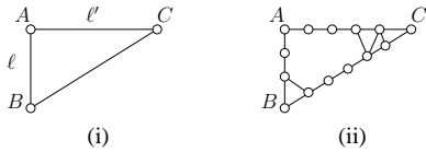
Figure 8. (i) An amplifier; (ii) The realization of an amplifier by unit-disk graphs.
