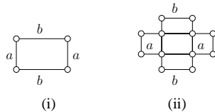
Figure 9. (i) Propagator; (ii) Crossing propagator.
